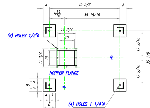
ANCHOR BOLT DETAIL
