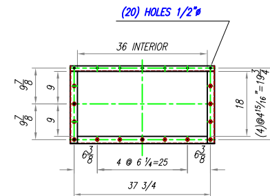
FLANGE DETAIL (CLEAN AIR OUTLET)
