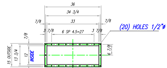
FLANGE DETAIL (DIRTY AIR INLET)
