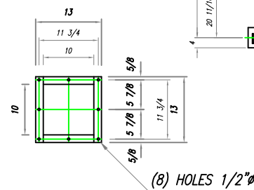
DETAIL B HOPPER FLANGE
