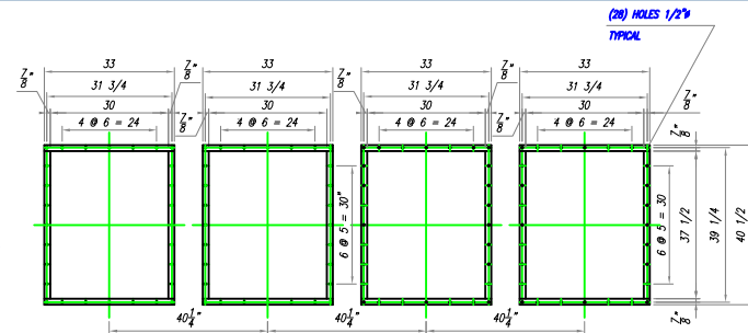
FLANGE DETAIL DIRTY AIR INLET
