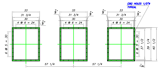
FLANGE DETAIL (DIRTY AIR INLET)
