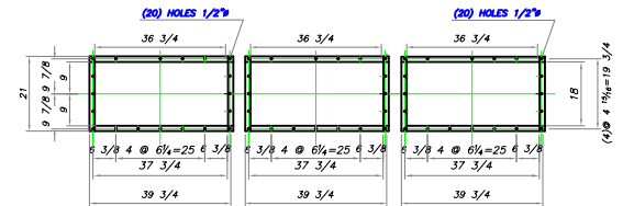
FLANGE DETAIL (CLEAN AIR OUTLET)
