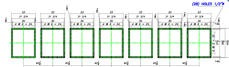
FLANGE DETAIL DIRTY AIR INLET
