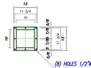
DETAIL B HOPPER FLANGE
