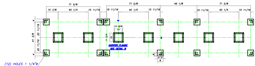
ANCHOR BOLT DETAIL
