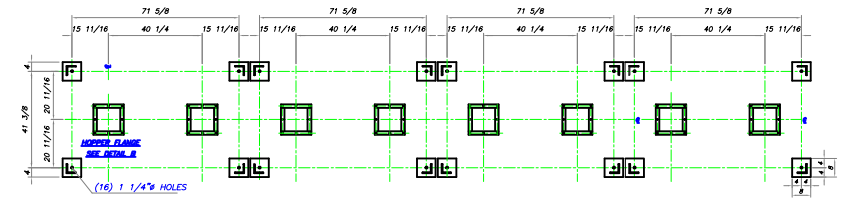
ANCHOR BOLT DETAIL
