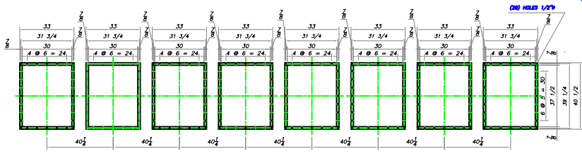
FLANGE DETAIL DIRTY AIR INLET
