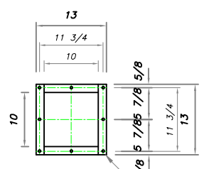
DETAIL B HOPPER FLANGE
