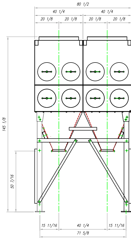
FRONT VIEW
