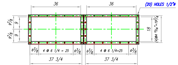
FLANGE DETAIL CLEAN AIR OUTLET
