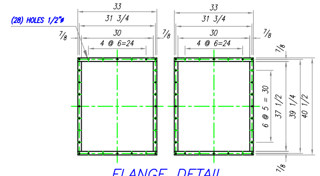
FLANGE DETAIL DIRTY AIR INLET
