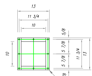
DETAIL B HOPPER FLANGE (8) HOLES 1/2"Ø
