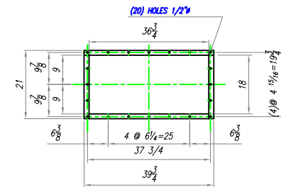
FLANGE DETAIL (CLEAN AIR OUTLET)
