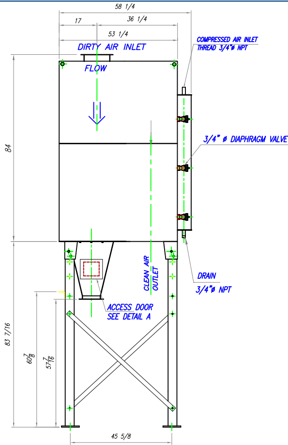
SIDE VIEW
