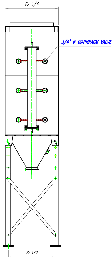
REAR VIEW
