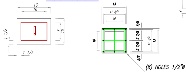
DETAIL A ACCESS DOOR
