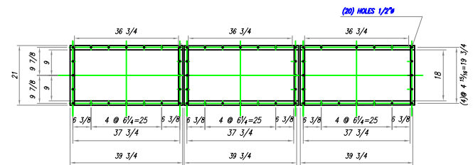
FLANGE DETAIL CLEAN AIR OUTLET
