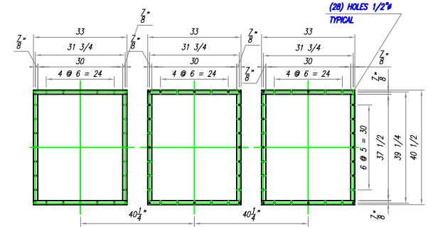
FLANGE DETAIL (DIRTY AIR INLET)
