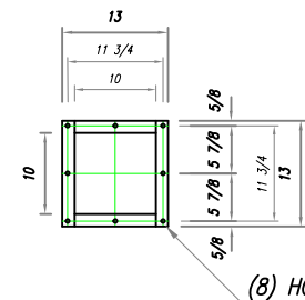
DETAIL B HOPPER FLANGE
