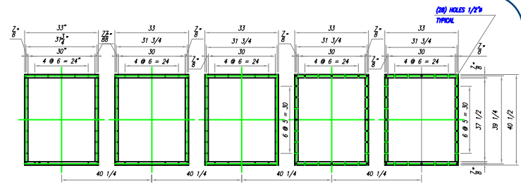
FLANGE DETAIL (DIRTY AIR INLET)
