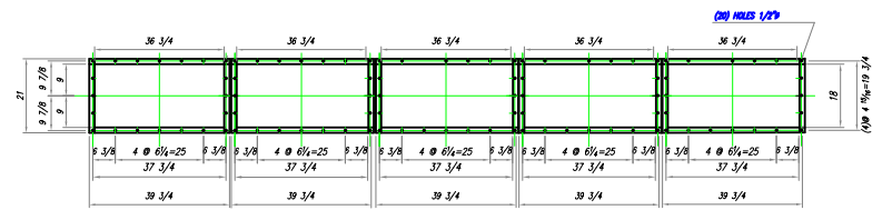
FLANGE DETAIL (CLEAN AIR OUTLET)
