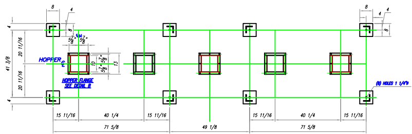
ANCHOR BOLT DETAIL
