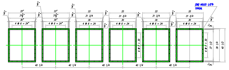
FLANGE DETAIL (DIRTY AIR INLET)
