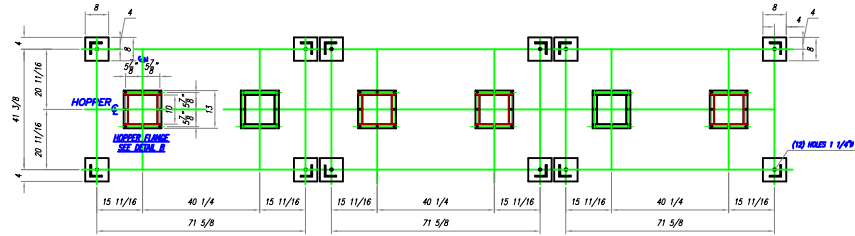
ANCHOR BOLT DETAIL
