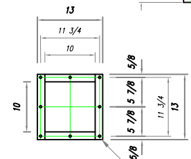
DETAIL B HOPPER FLANGE
