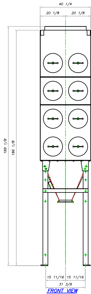
FRONT VIEW
