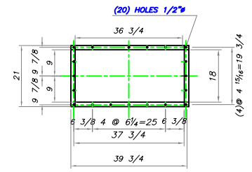
FLANGE DETAIL CLEAN AIR OUTLET
