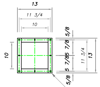
DETAIL B HOPPER FLANGE (8) HOLES 1/2"Ø
