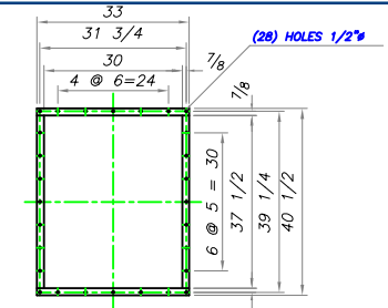
FLANGE DETAIL DIRTY AIR INLET
