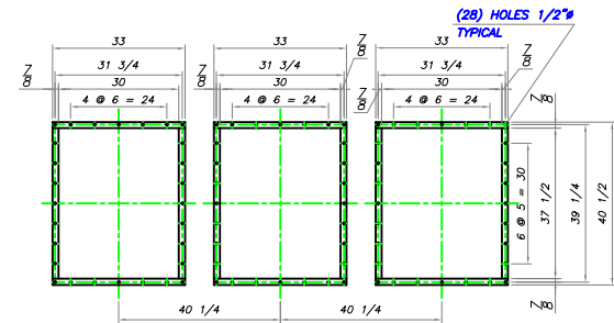
FLANGE DETAIL DIRTY AIR INLET
