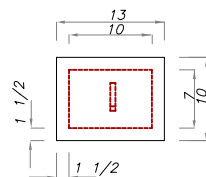
DETAIL A ACCESS DOOR
