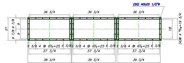
FLANGE DETAIL CLEAN AIR OUTLET
