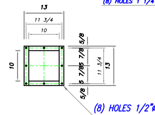
DETAIL B HOPPER FLANGE
