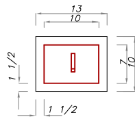
DETAIL A ACCESS DOOR
