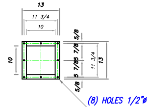
DETAIL B HOPPER FLANGE
