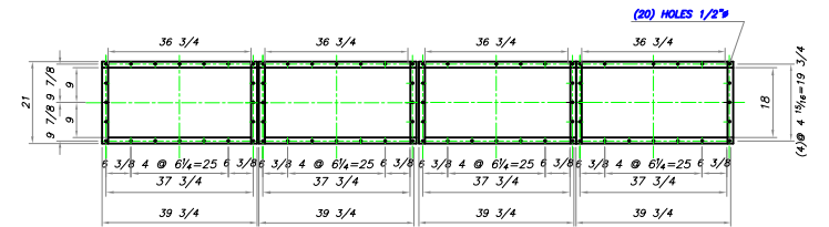
FLANGE DETAIL CLEAN AIR OUTLET
