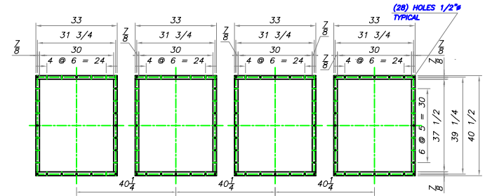
FLANGE DETAIL DIRTY AIR INLET
