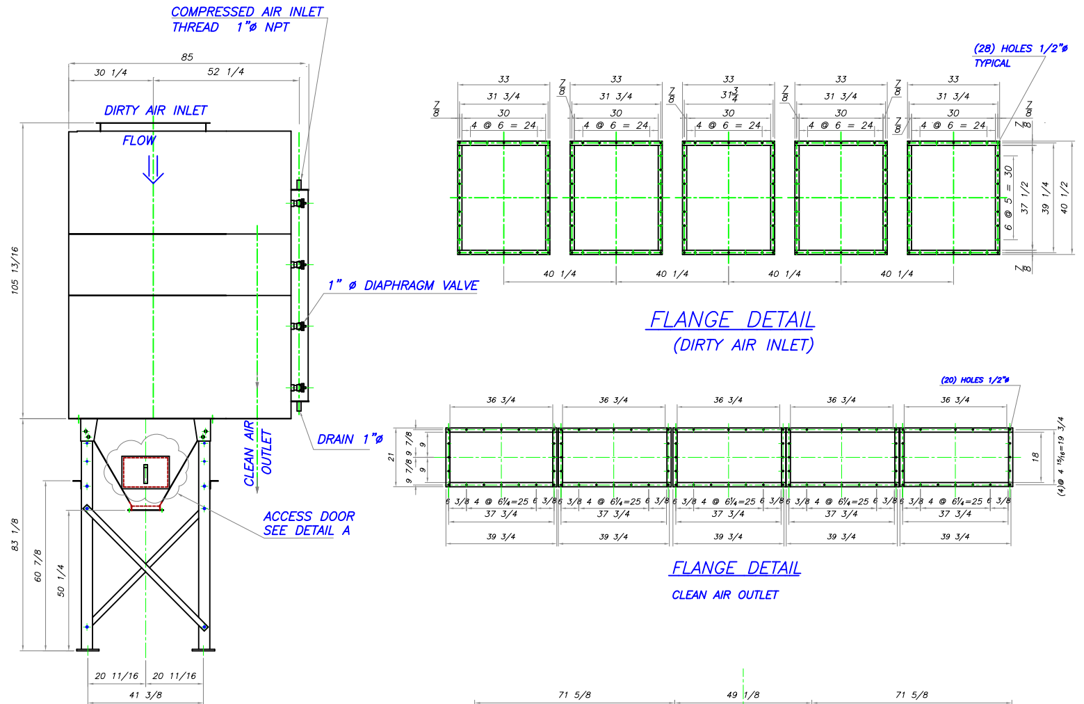
SIDE VIEW
