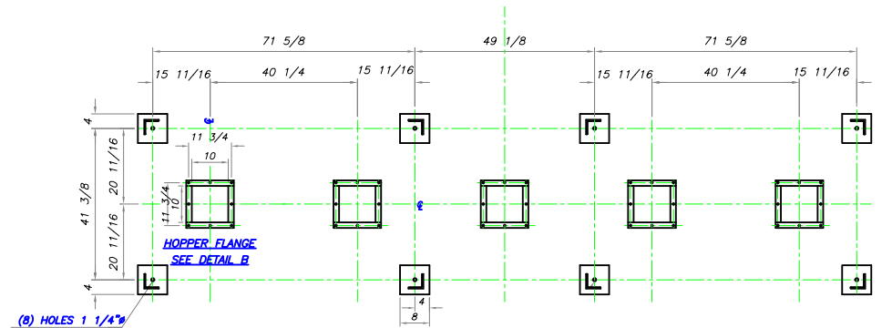
ANCHOR BOLT DETAIL
