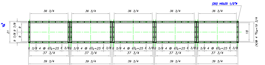
FLANGE DETAIL CLEAN AIR OUTLET
