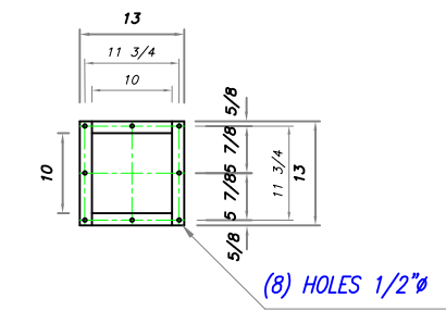
DETAIL B HOPPER FLANGE
