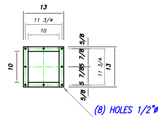
DETAIL B HOPPER FLANGE
