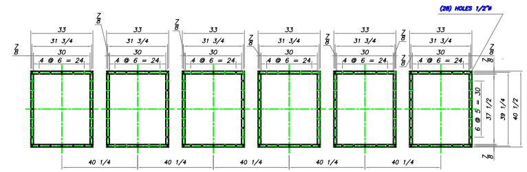
FLANGE DETAIL (DIRTY AIR INLET)
