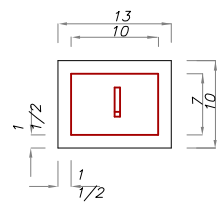
DETAIL A ACCESS DOOR
