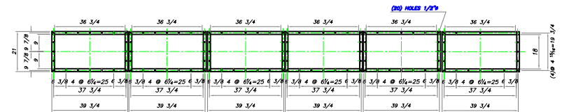
FLANGE DETAIL (CLEAN AIR OUTLET)
